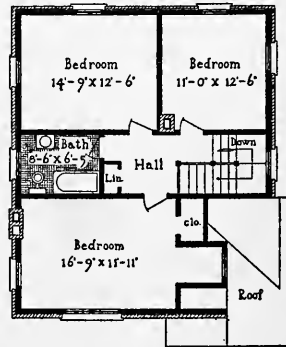
Second-floor Plan
